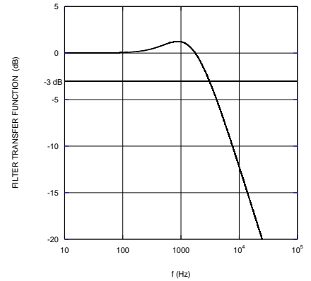
Filter Transfer Function
