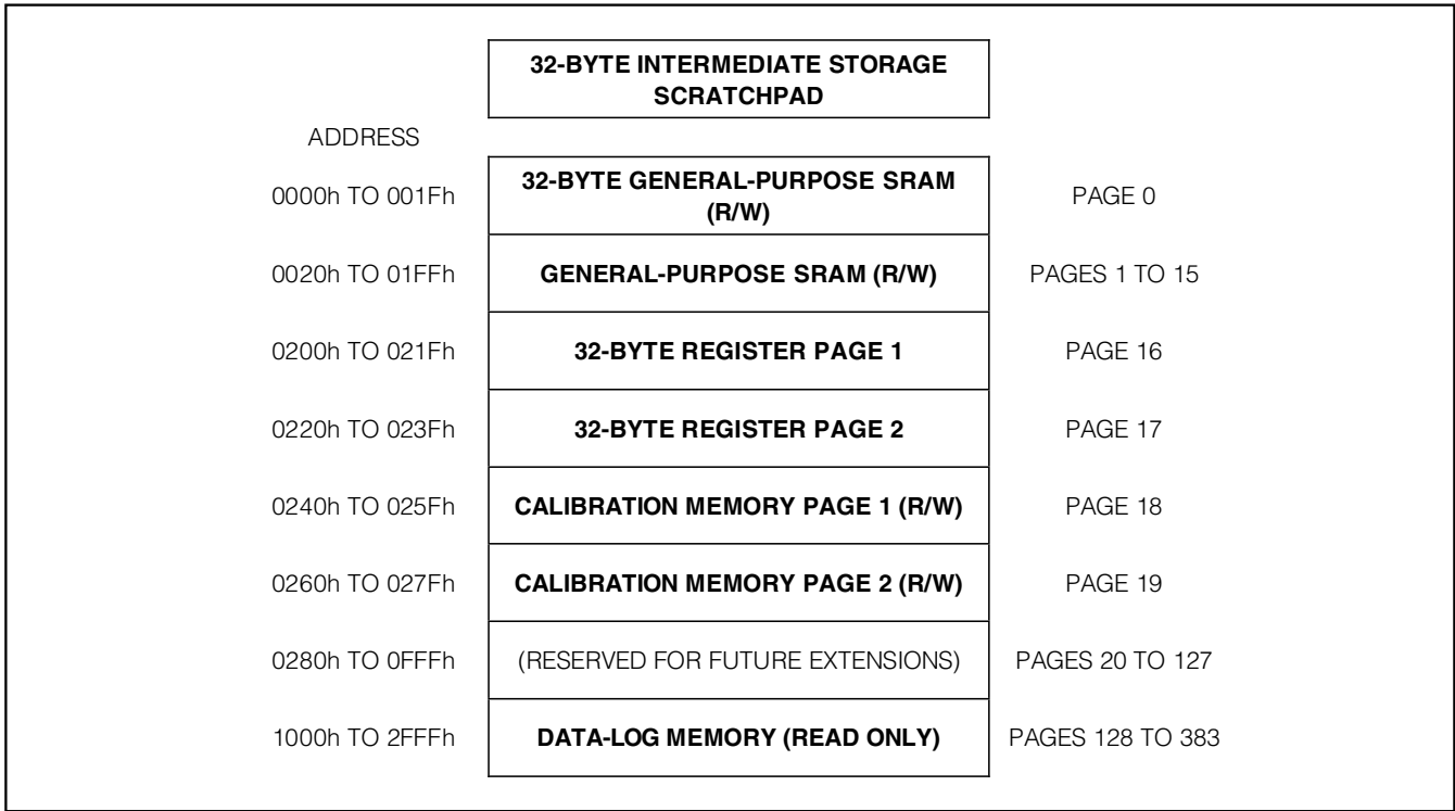
Figure 5. Memory Map
