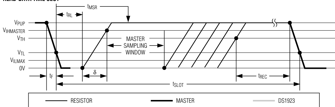
Figure 13. Read/Write Timing Diagrams
