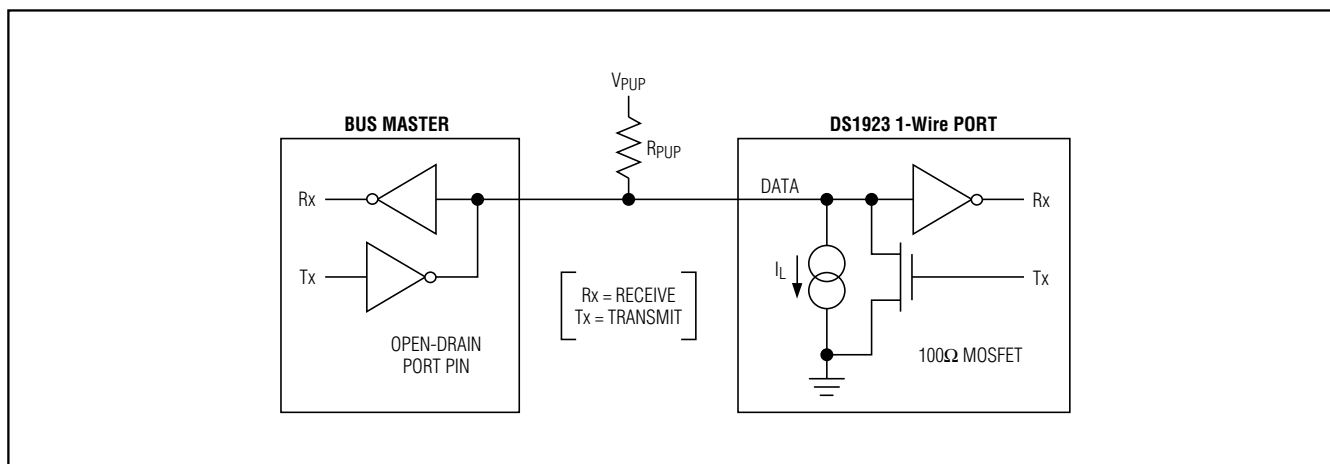
Figure 10. Hardware Configuration
