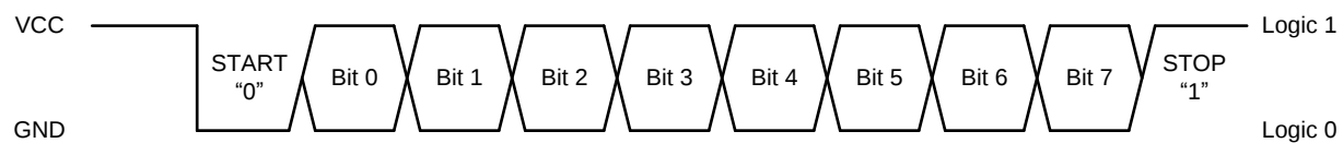
Figure 28. UART 8 – 1 Signaling
