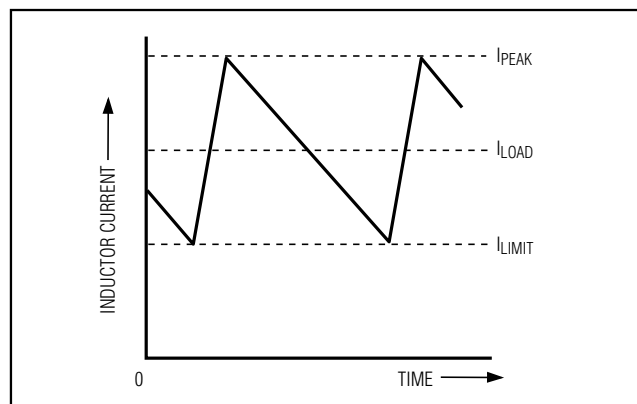
Figure 4. “Valley” Current-Limit Threshold Point
