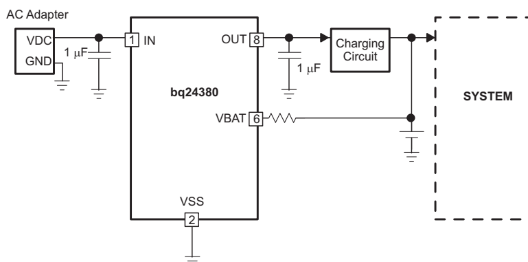
Simplified Schematic
