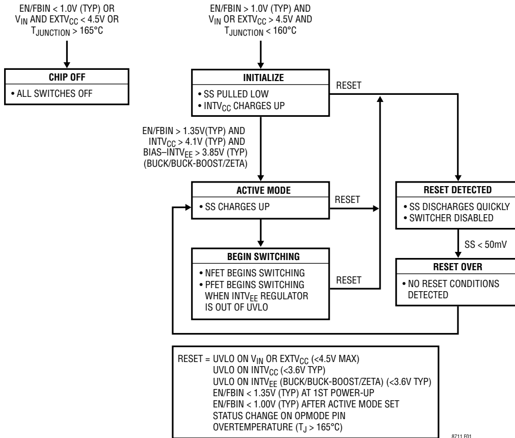
Figure 1. State Diagram
