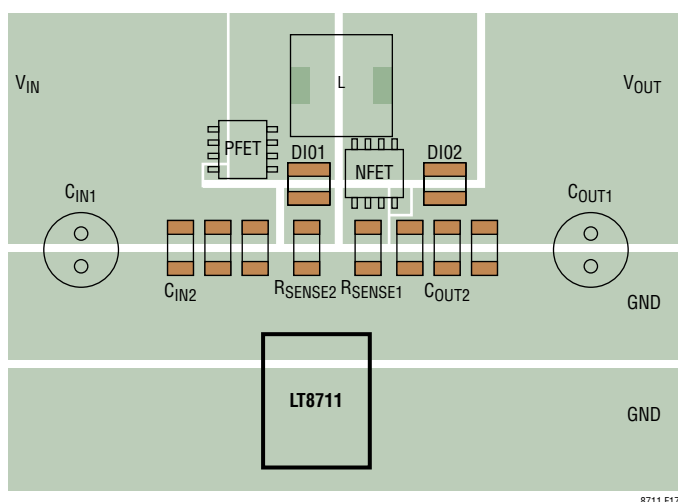
Figure 17. Suggested Component Placement for Buck-Boost Topology
