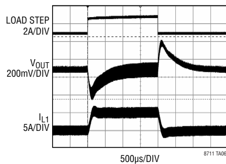
Transient Response with 1.5A to 3A to 1.5A Output Load Step (VIN = 9V)
