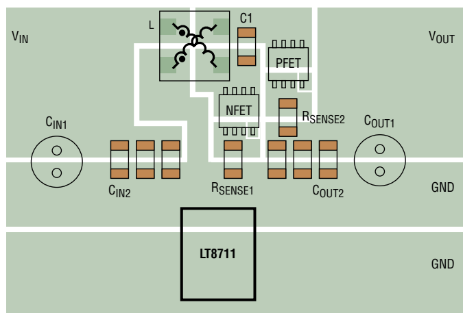
Figure 15. Suggested Component Placement for SEPIC Topology
