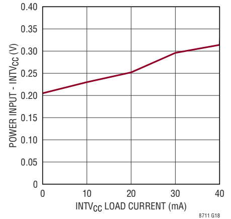
INTV CC Dropout from V_{IN} or V_{EXTVCC}
