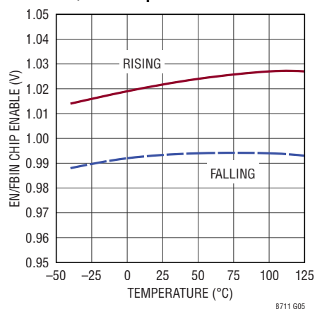
EN/FBIN Chip Enable Threshold
