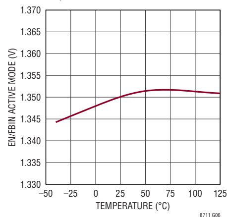
EN/FBIN Active Mode Threshold
