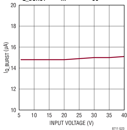
I Q_BURST vs V IN or EXT VCC
