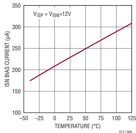
ISN Bias Current
