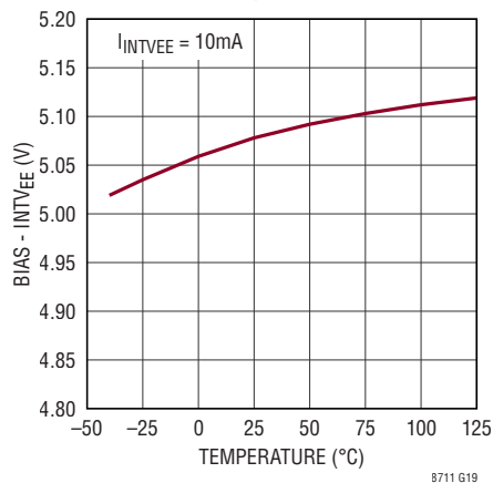
INTV EE vs Temperature
