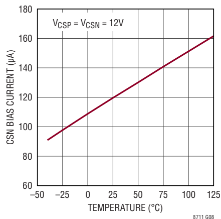
CSN Bias Current
