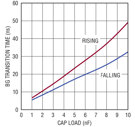
BG Transition Time vs Cap Load
