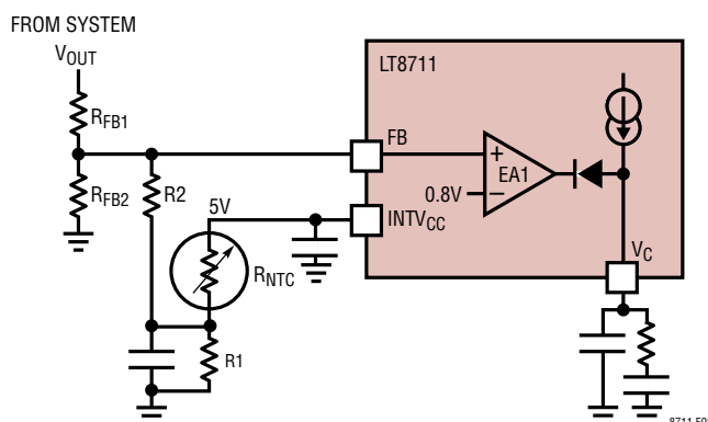
Figure 8. Temperature Dependent Output Using an NTC Resistor Divider
