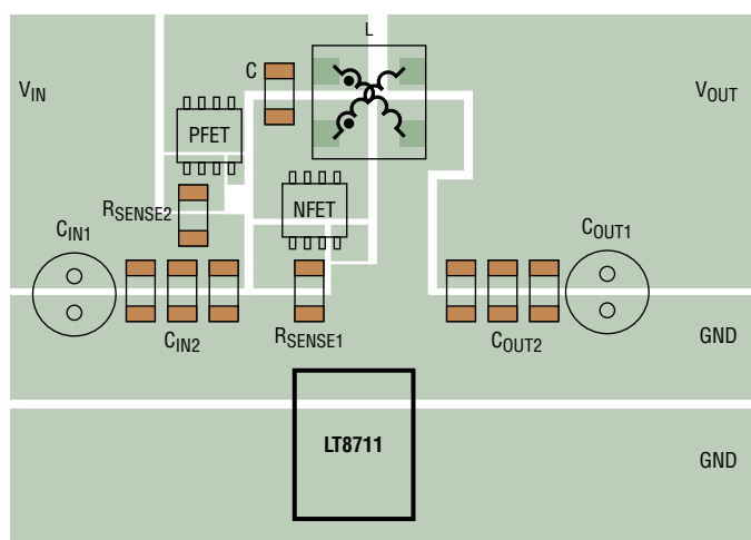
Figure 16. Suggested Component Placement for ZETA Topology
