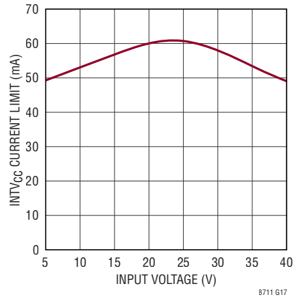
INTV CC Current Limit vs V_{IN} or V_{EXTVCC}
