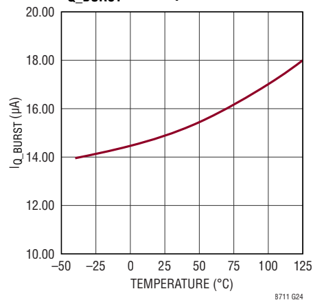
I Q_BURST vs Temperature
