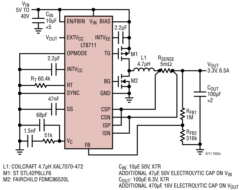
400kHz, 5V–40V Input to 3.3V/6.5A Buck
