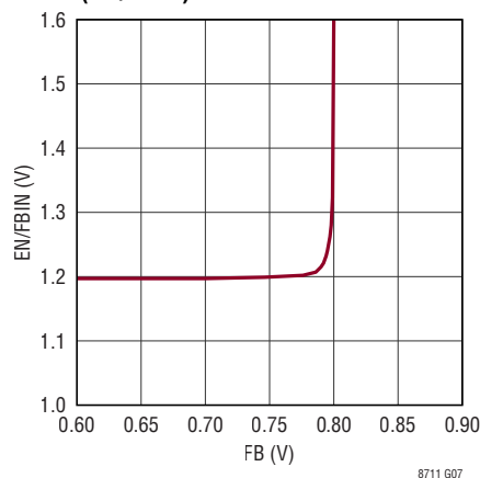
Input Voltage Regulation vs FB (EN/FBIN)
