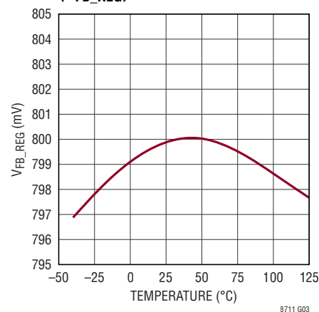
Output Voltage Regulation ( V_{FB\_REG} )
