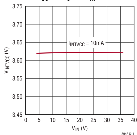
INTV CC Voltage vs V IN
