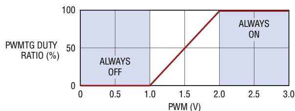
Figure 13. Internal PWM Dimming Duty Ratio vs PWM Voltage
