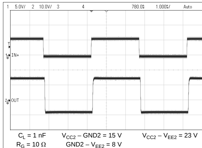
Figure 52. Normal Operation - Bipolar Supply
