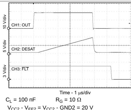
Figure 15. Output Transient Waveform DESAT and \overline{FLT}
