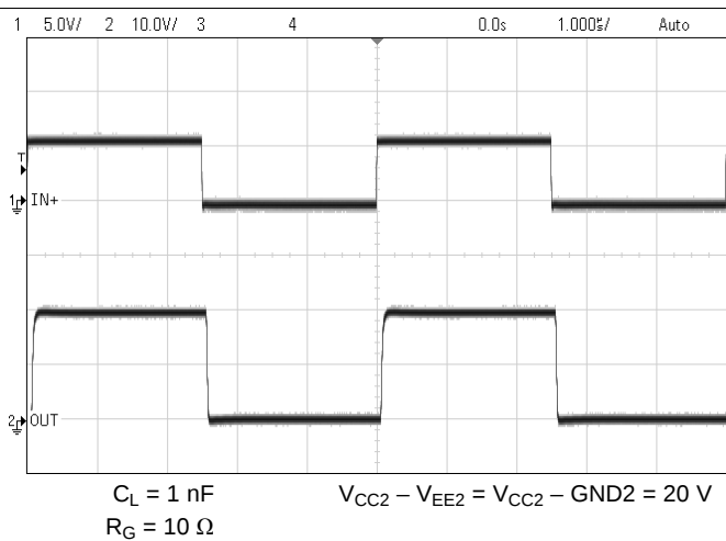
Figure 53. Normal Operation - Unipolar Supply
