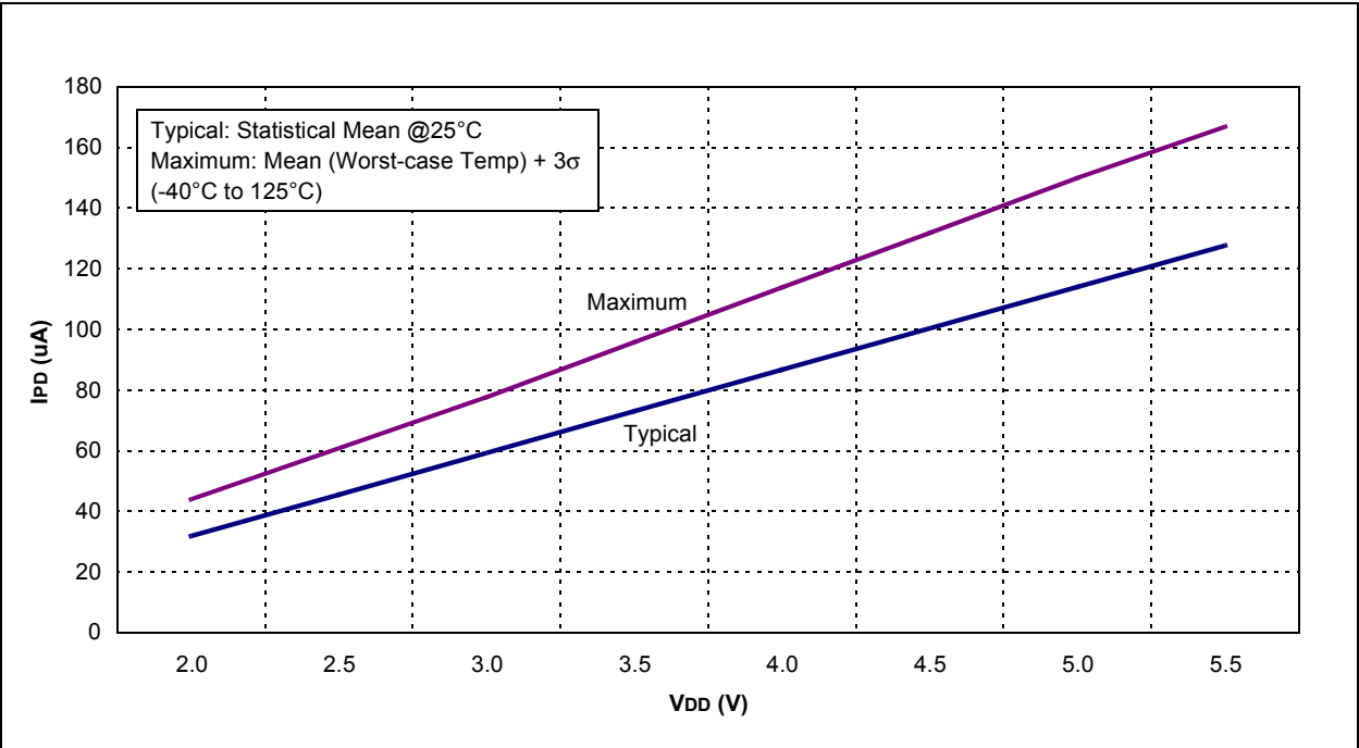
FIGURE 20-15: COMPARATOR I PD vs. V DD (BOTH COMPARATORS ENABLED)
