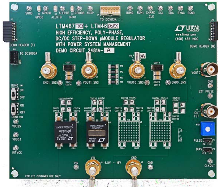
Figure 1. LTM4677 + LTM4650; 86A DC2481A-A Demo Circuit
