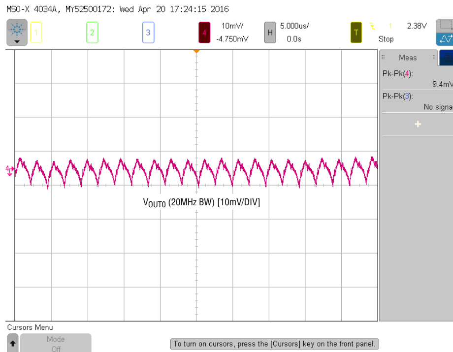
Figure 7. Output Voltage Ripple at V_{IN} = 12V , V_{OUT0} = 1V , I_{OUT0} = 86A
