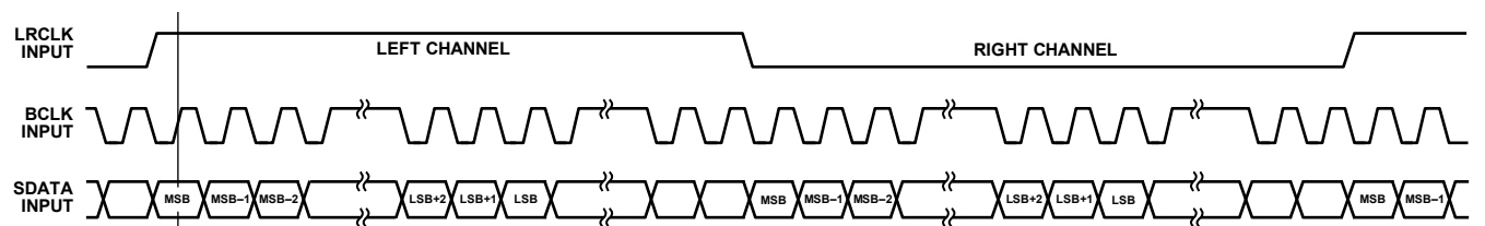
Figure 5. Left-Justified Mode
