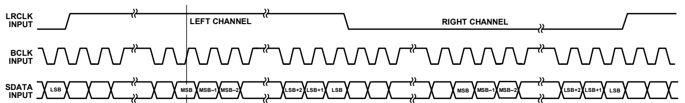
Figure 3. Right-Justified Mode
