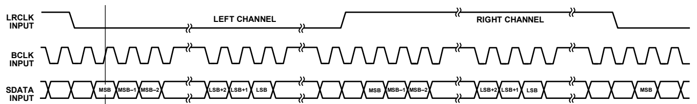
Figure 4. I 2 S-Justified Mode
