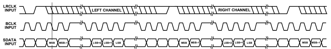
Figure 6. Left-Justified DSP Mode
