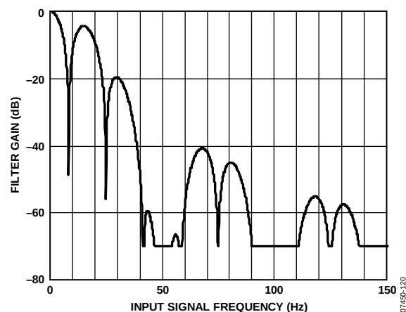
Figure 20. Capacitance Channel Frequency Response, Conversion Time = 60 ms
