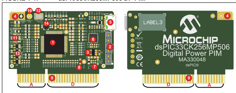
FIGURE 1-1: dsPIC33CK256MP506 DP PIM
