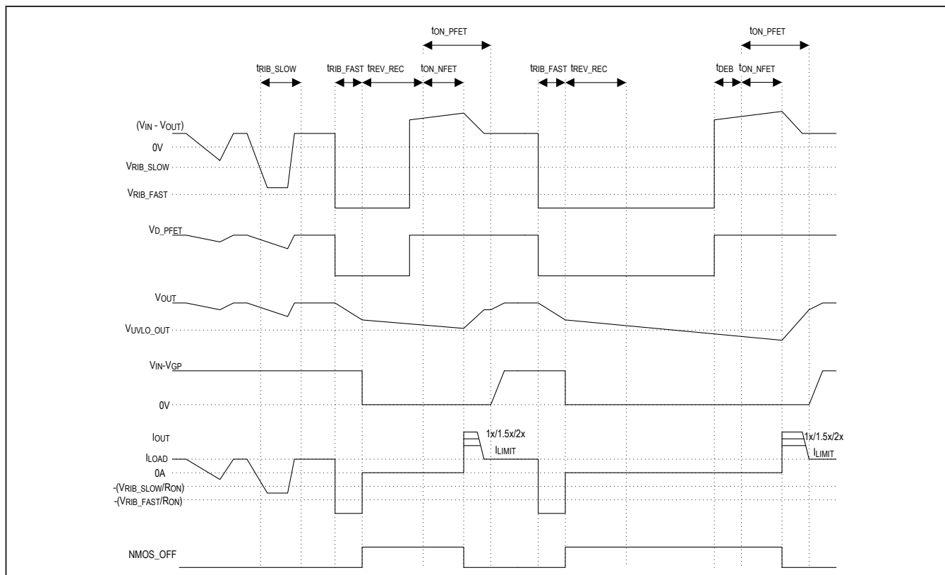
Figure 7. Fast Reverse-Current Fault Timing Diagram
