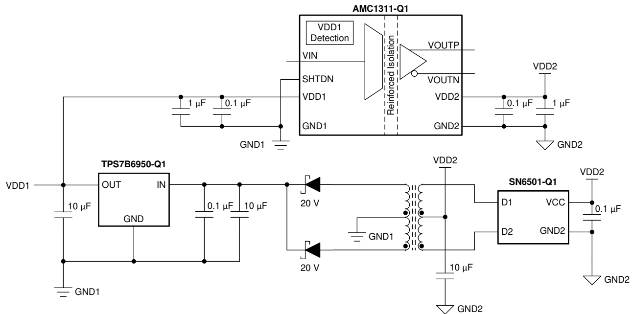
Figure 52. SN6501-Q1-Based, High-Side Power Supply
