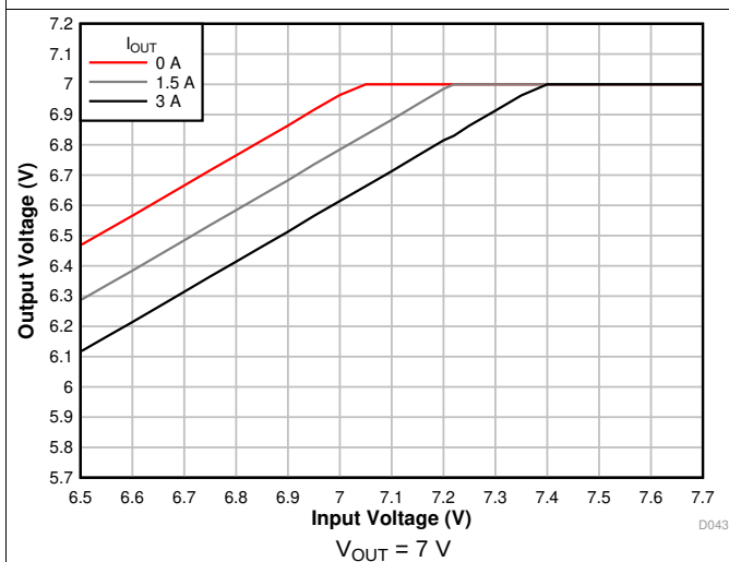
Figure 35. Voltage Dropout
