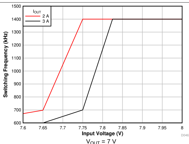
Figure 36. Frequency Foldback
