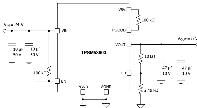
Figure 40. TPSM53603 Typical Schematic
