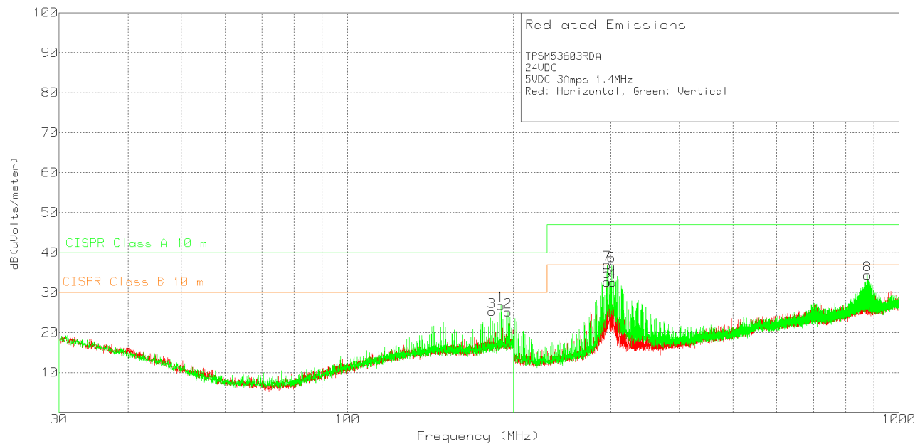
Figure 48. Radiated Emissions 24-V Input, 5-V Output, 3-A Load
