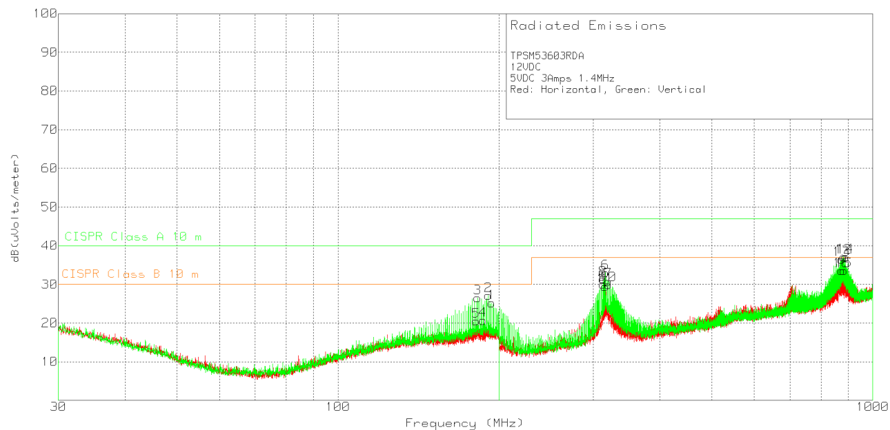
Figure 49. Radiated Emissions 12-V Input, 5-V Output, 3-A Load
