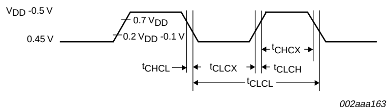
Fig 15. Clock signal waveform for I_{CC} tests in active and idle modes ( t_{CLCH} = t_{CHCL} = 5 ns).
