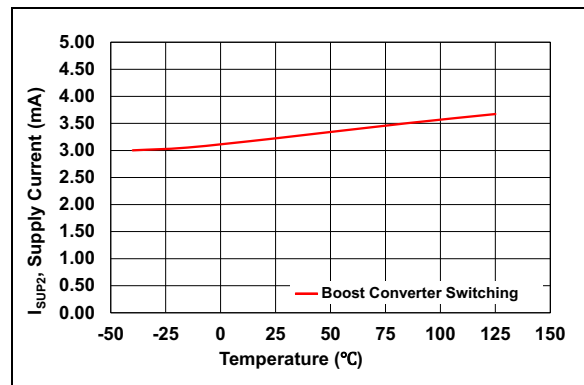
FIGURE 2-5: Supply Current vs. Temperature (Boost Converter Switching).
