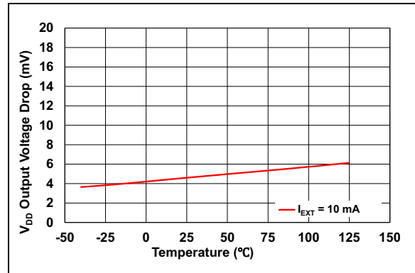
FIGURE 2-4: V_{DD} Output Voltage Drop vs. Temperature.
