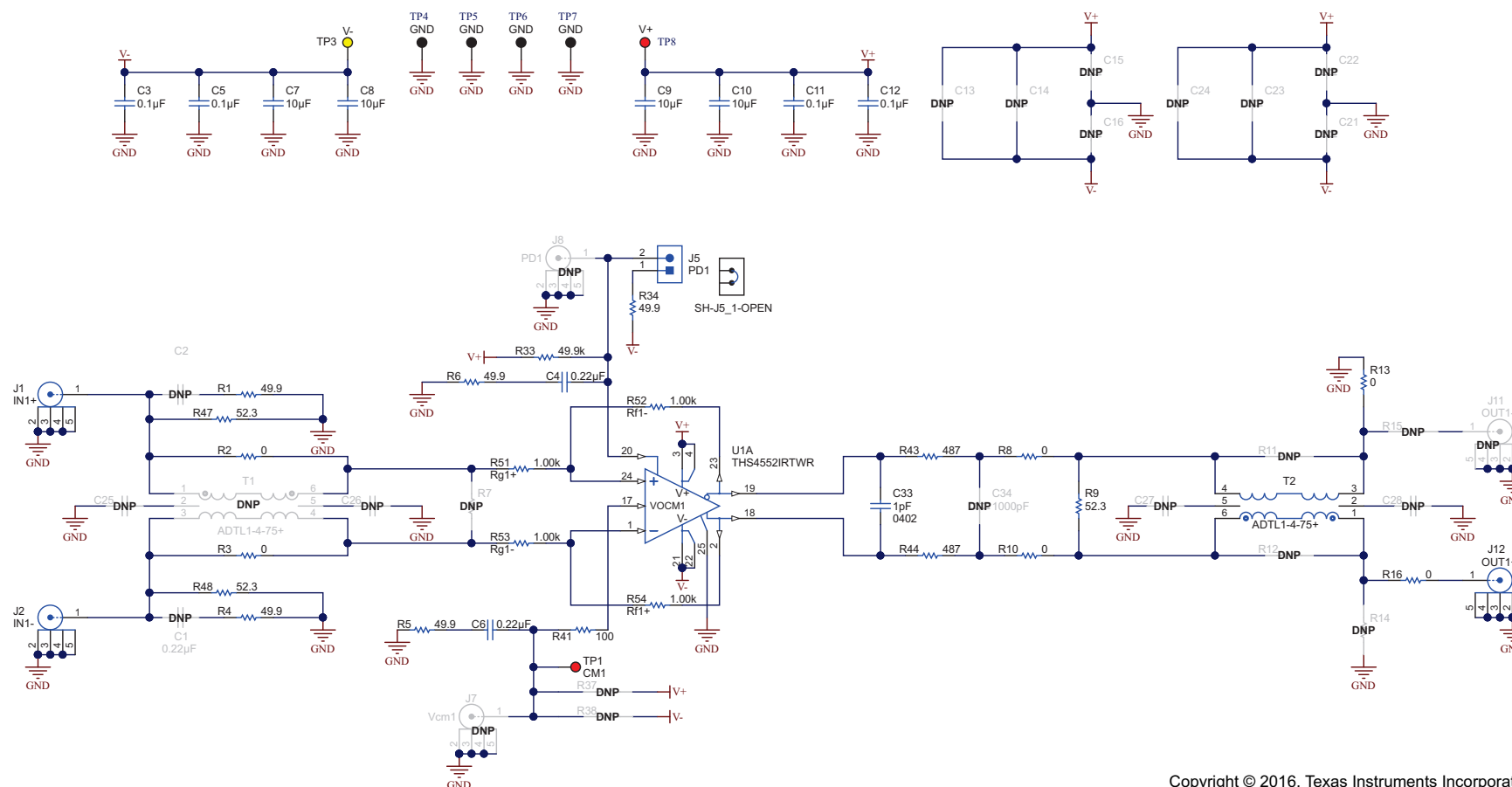
Figure 1. THS4552RTWEVM Schematic
