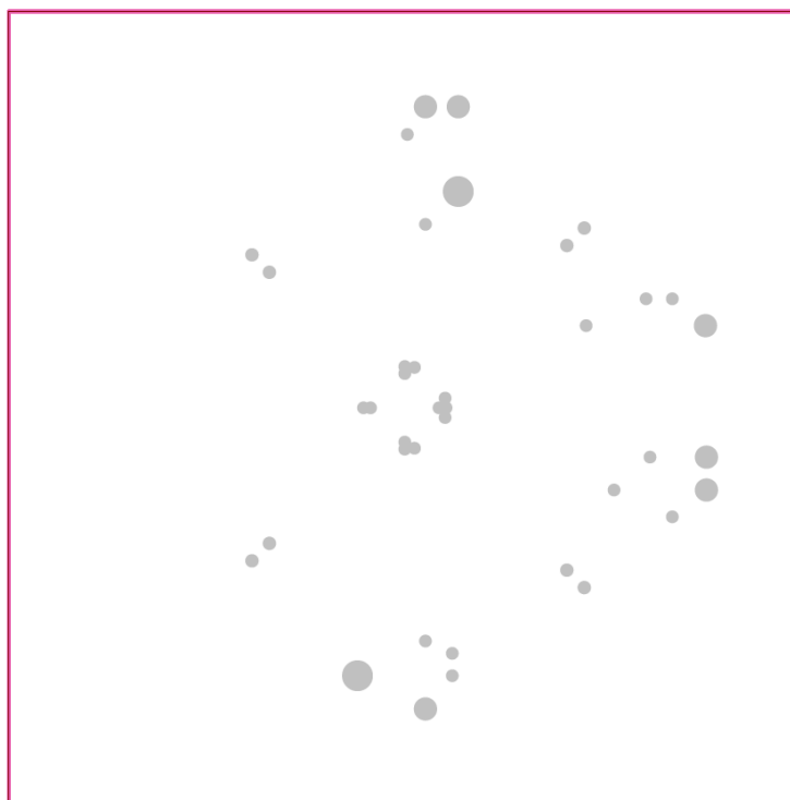
Figure 5. THS4552RTWEVM Layer 3
