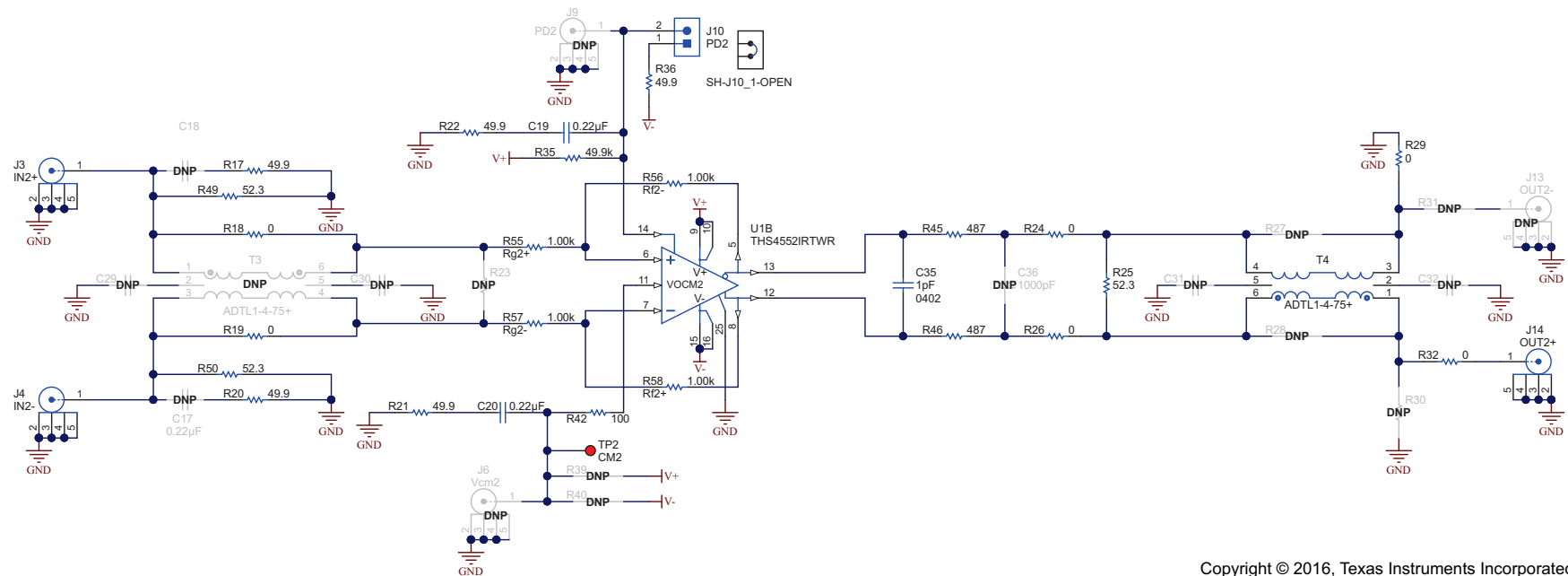
Figure 2. THS4552RTWEVM Schematic
