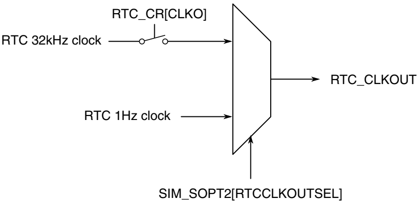
Figure 3-41. RTC_CLKOUT generation
