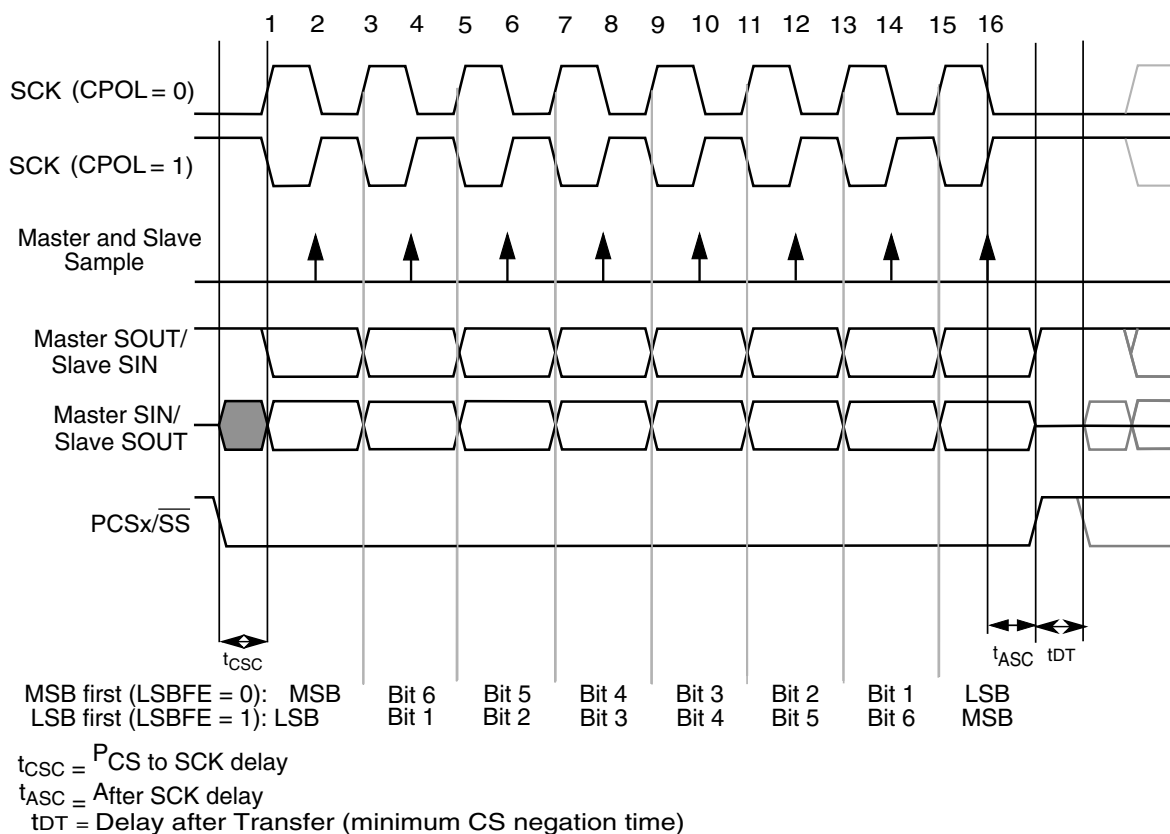
Figure 41-50. Module transfer timing diagram (MTFE=0, CPHA=1, FMSZ=8)
