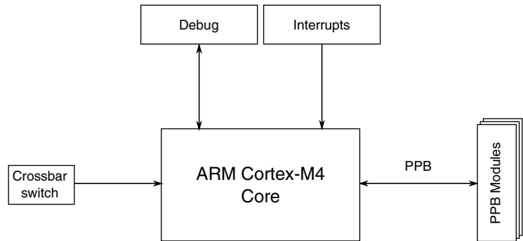
Figure 3-1. Core configuration
