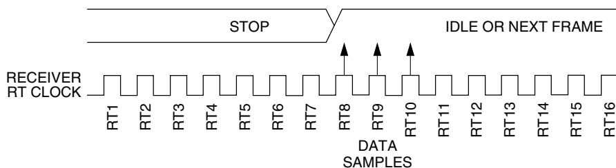
Figure 43-168. Fast data
