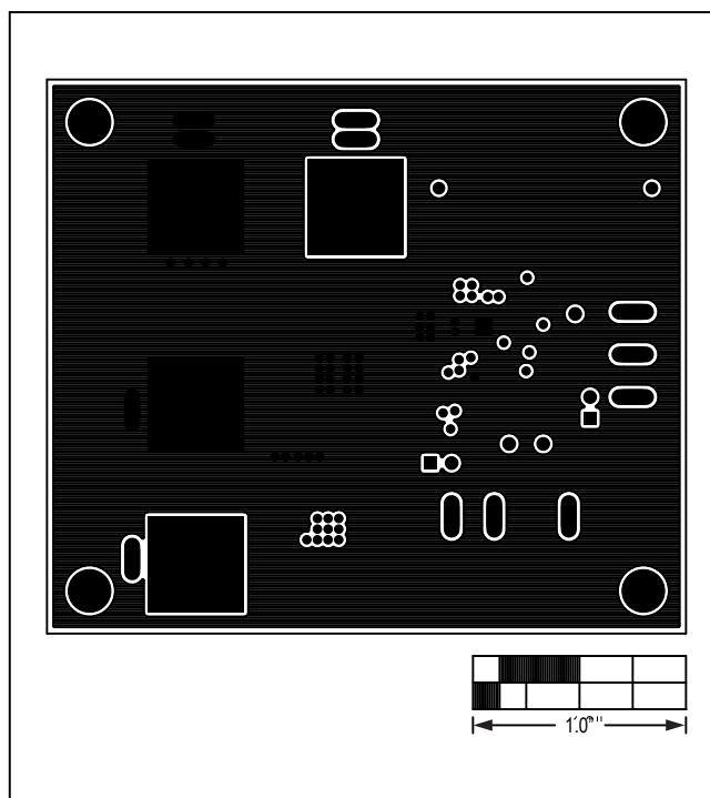
Figure 6. MAX16962R EV Kit PCB Layout—Solder Side
