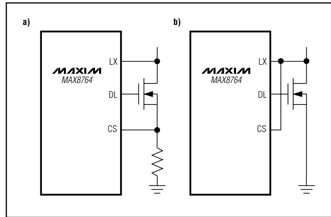
Figure 8. Current-Sense Circuits
