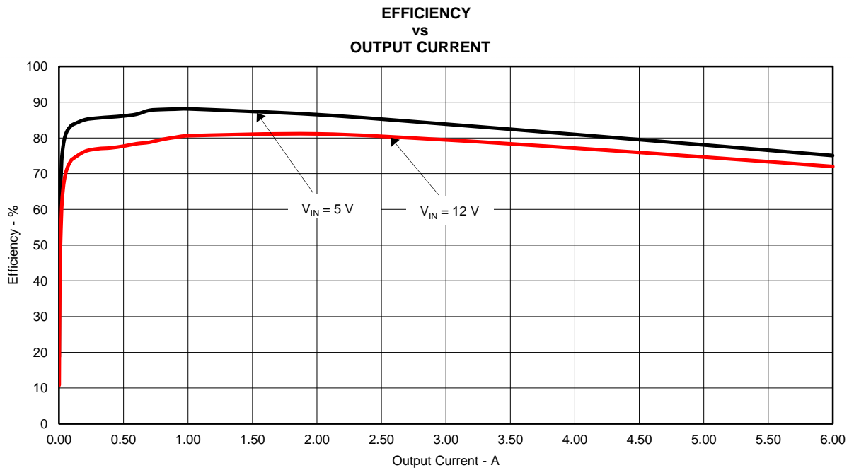
Figure 1. TPS56628EVM-534 Efficiency
