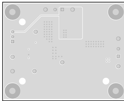
Figure 17. Internal Layer 2
