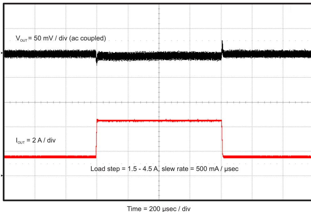
Figure 5. TPS56628EVM-534 Load Transient Response
