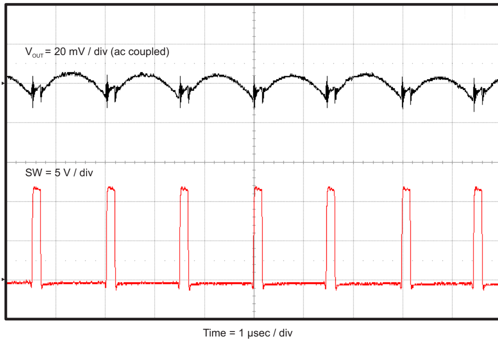
Figure 6. TPS56628EVM-534 Output Voltage Ripple ( I_{OUT} = 6 \text{ A} )
