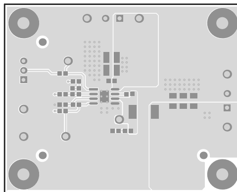
Figure 15. Top Layer
