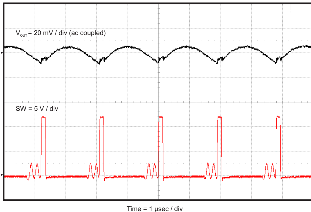
Figure 7. TPS56628EVM-534 Output Voltage Ripple ( I_{OUT} = 500 \text{ mA} )
