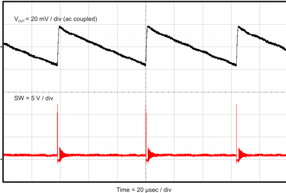
Figure 8. TPS56628EVM-534 Output Voltage Ripple ( I_{OUT} = 10 \text{ mA} )
