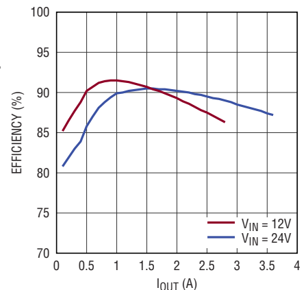
Efficiency with V_{OUT} = -5V
