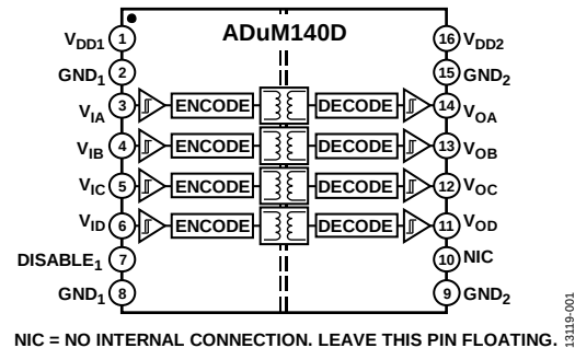
Figure 1. ADuM140D Functional Block Diagram
