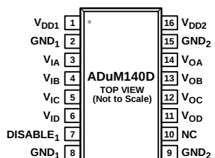
Figure 4. ADuM140D Pin Configuration
