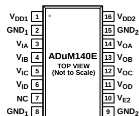
Figure 5. ADuM140E Pin Configuration
