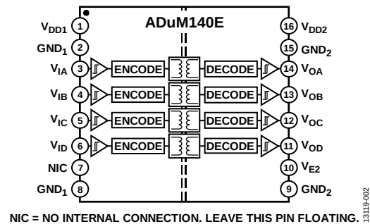
Figure 2. ADuM140E Functional Block Diagram
