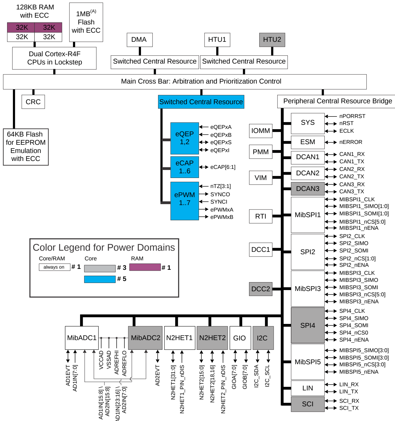
Figure 1-1. Functional Block Diagram (B)
