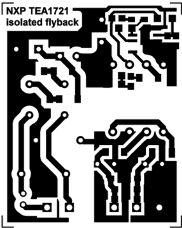
b. Bottom copper and bottom silk screen plus component placement
