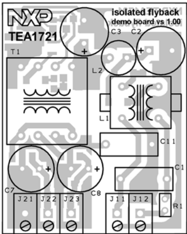
a. Top silk screen plus top component placement and drill pattern
