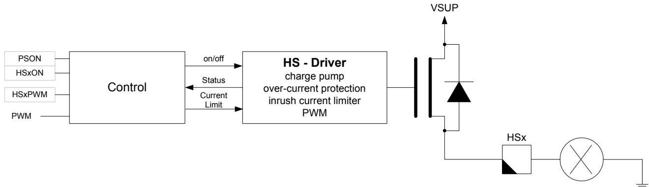
Figure 23. HS Circuitry
