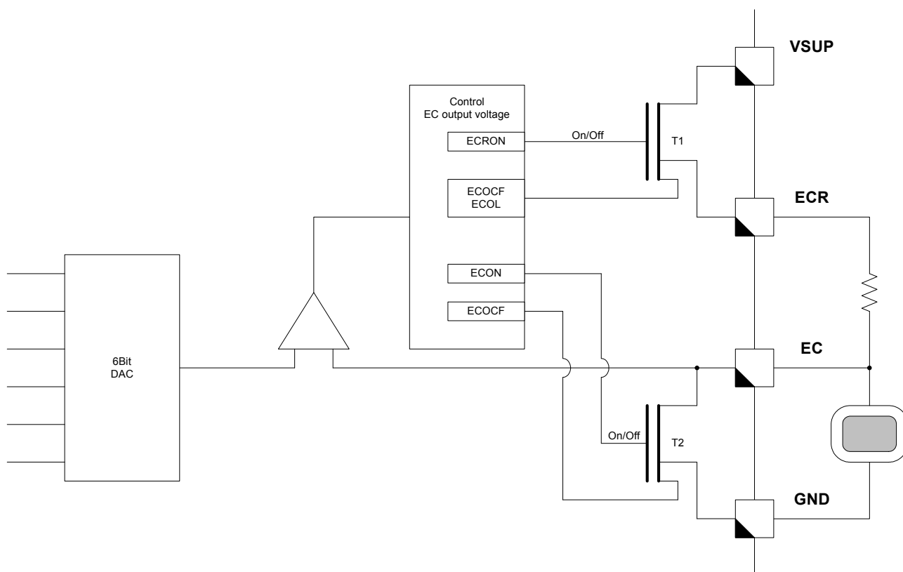
Figure 25. EC Circuitry
