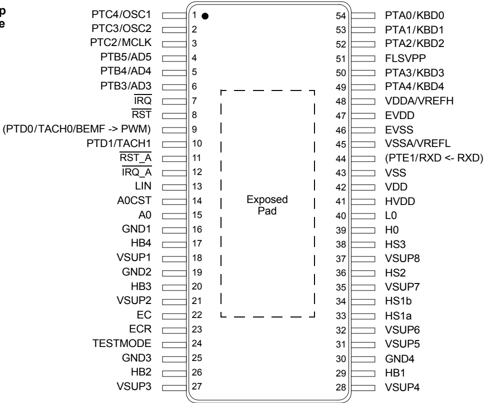
Figure 3. Pin Connections
