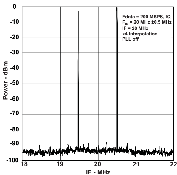
Figure 8. Two Tone IMD Spectral Plot
