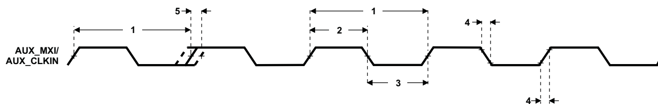
Figure 7-16. AUX_MXI/AUX_CLKIN Timing
