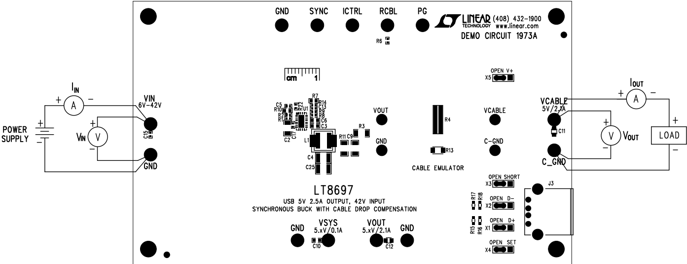
Figure 2. Proper Measurement Equipment Setup
