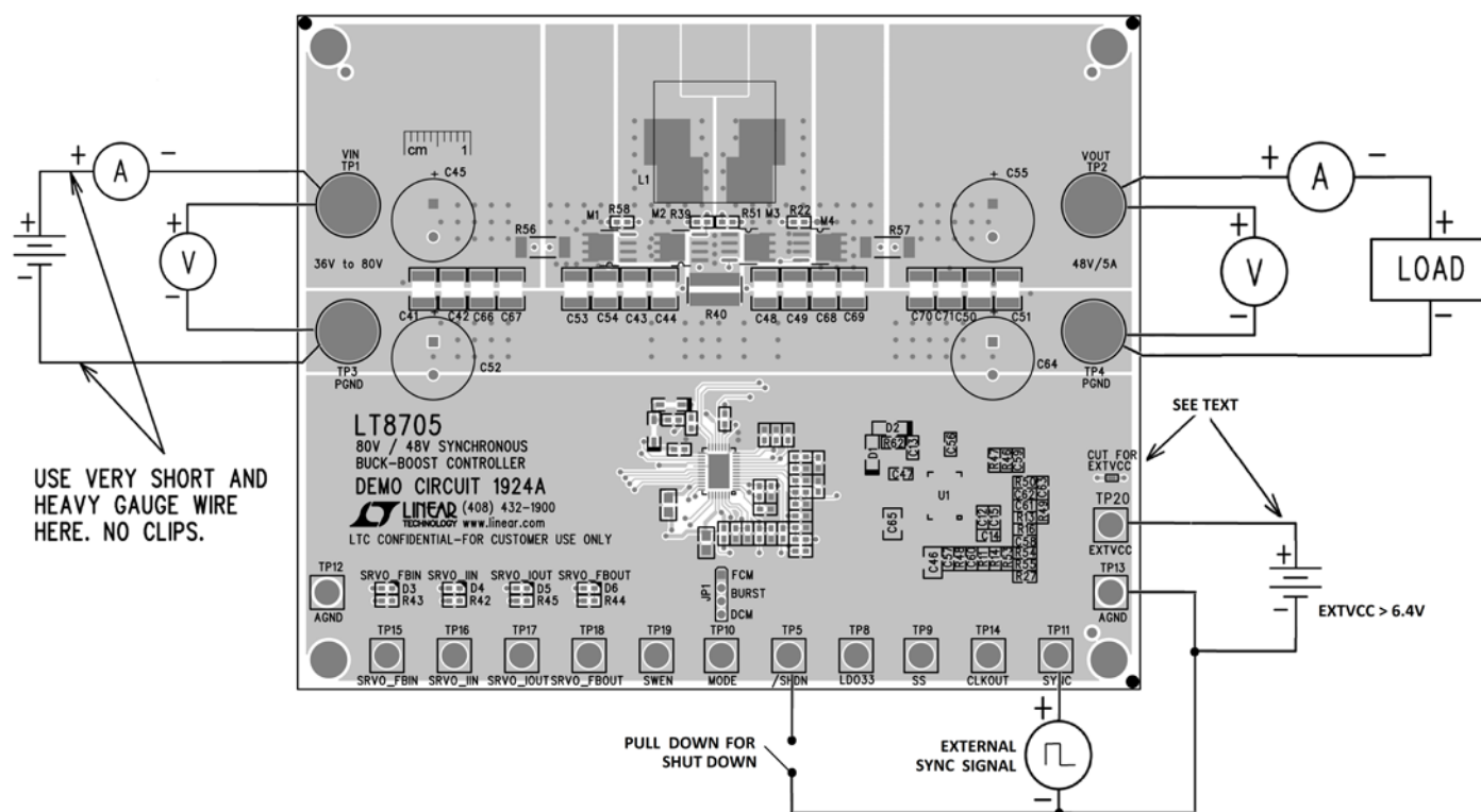
Figure 2. Test Setup
