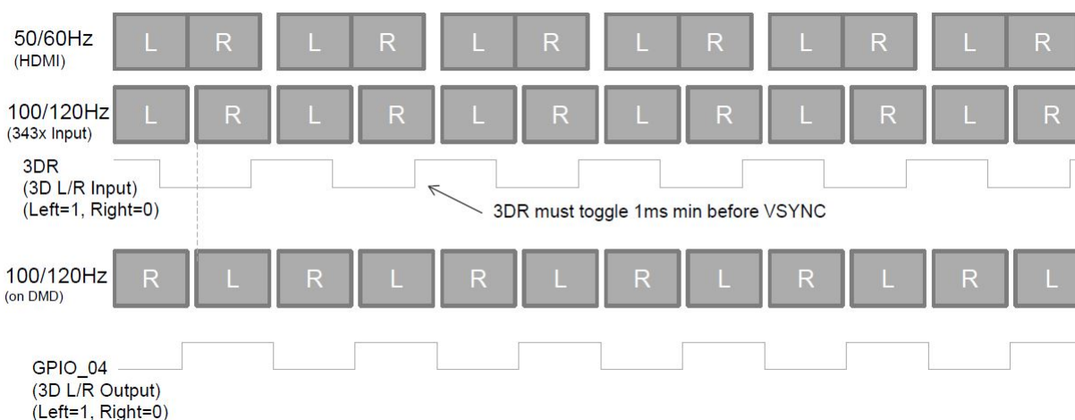
Figure 11. DLPC343x L/R Frame and Signal Timing
