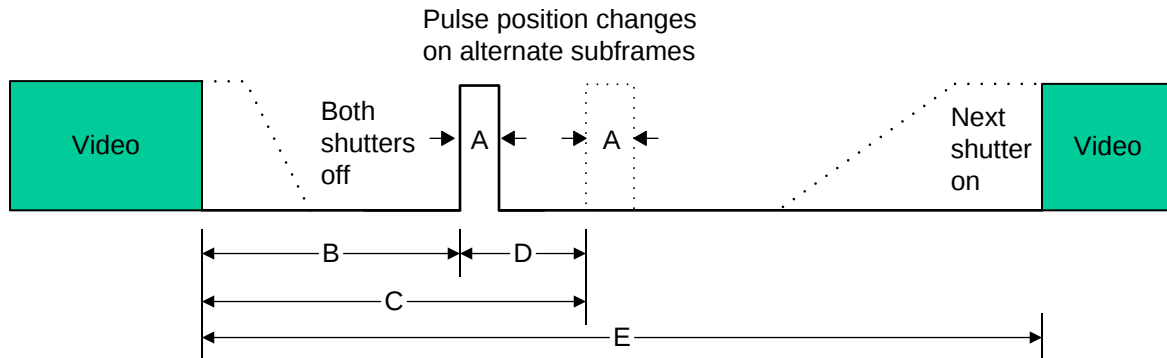
Figure 24. 3D DLP Link Pulse Timing
