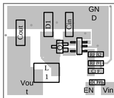
Figure 4. Top Side Layout
