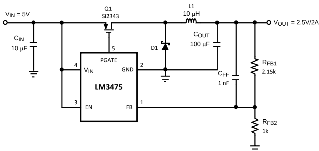
Figure 1. Full Demo Board Schematic
