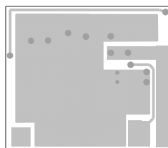
Figure 5. Bottom Side Layout
