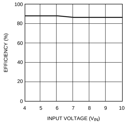
Figure 3. Efficiency vs Input Voltage ( I_{OUT} = 2\text{ A} )
