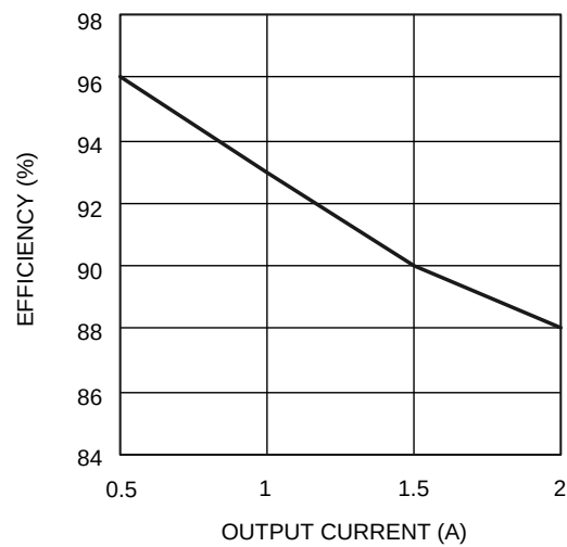
Figure 2. Efficiency vs Output Current ( V_{IN} = 5\text{ V} )
