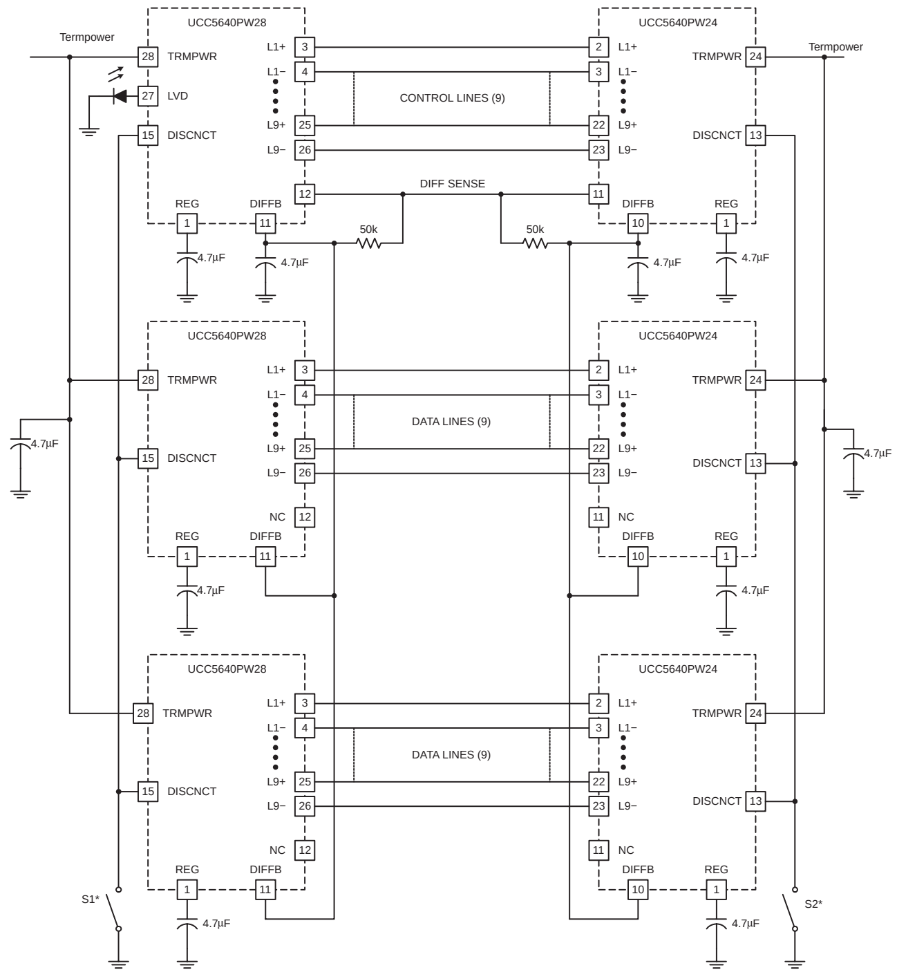
Figure 1. Application Diagram
