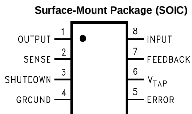
Figure 4. Top View
