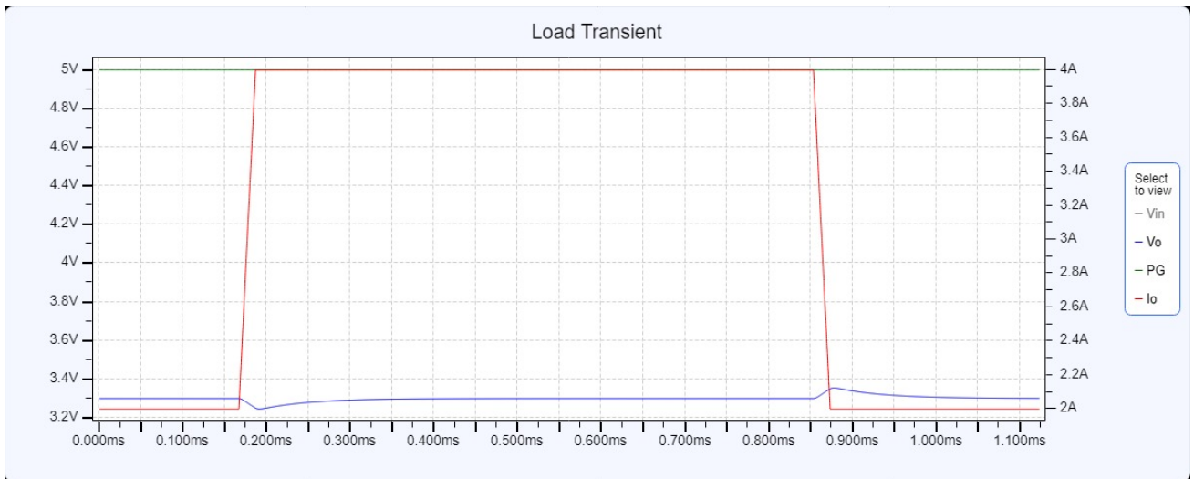
Vin = 6V, Ihigh = 4A, Ilow = 2A, Slew rate = 0.1A/μs
