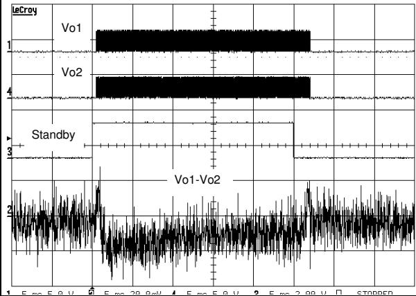
Figure 60. Startup and shutdown time V_{CC} = 3\text{ V} , G = 6\text{ dB} , C_{in} = 100\text{ nF} (5 ms/div)
