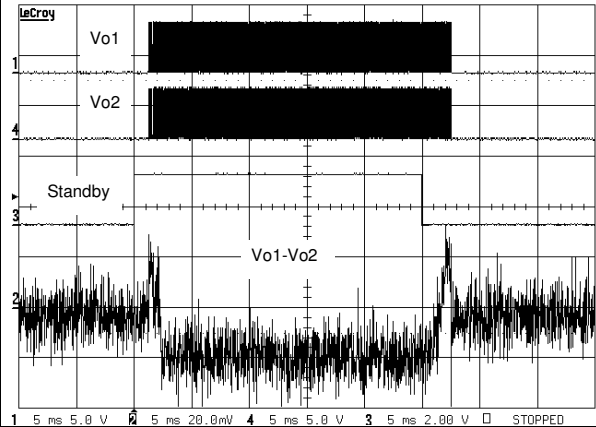
Figure 61. Startup and shutdown time V_{CC} = 5\text{ V} , G = 6\text{ dB} , No C_{in} (5 ms/div)
