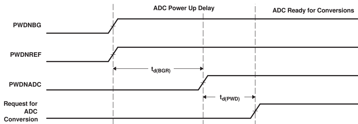
Figure 5-20. ADC Power-Up Control Bit Timing
