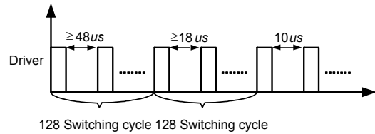
Figure 2— \tau_{\text{minoff}} at start-up
