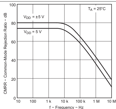
Figure 25. Common-Mode Rejection Ratio vs Frequency
