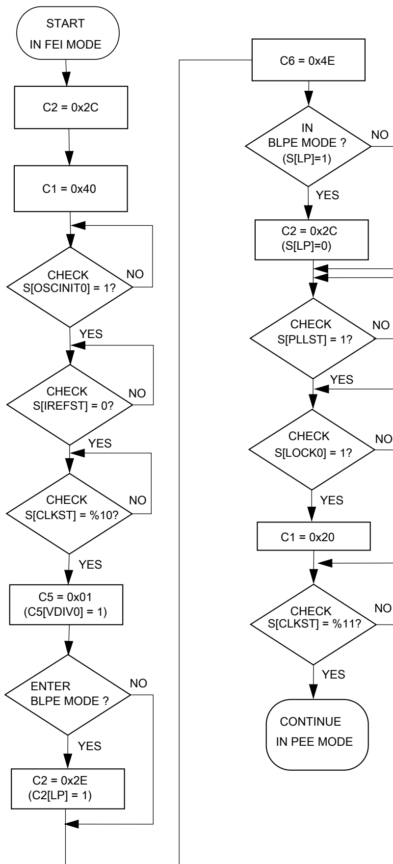
Figure 28-3. Flowchart of FEI to PEE mode transition using an 16 MHz crystal Kinetis K28F MCU Sub-Family Reference Manual, Rev. 4, 08/2017
