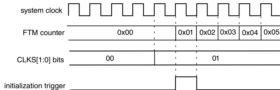
Figure 44-85. Initialization trigger is generated if (CNT = CNTIN), (CLKS[1:0] = 0:0), and a value different from zero is written to CLKS[1:0] bits
