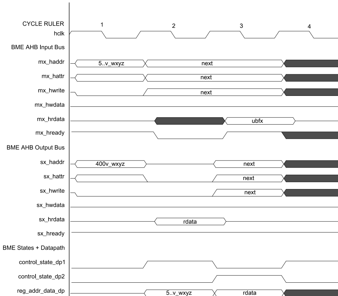
Figure 23-7. Decorated load: unsigned bit field insert timing diagram
