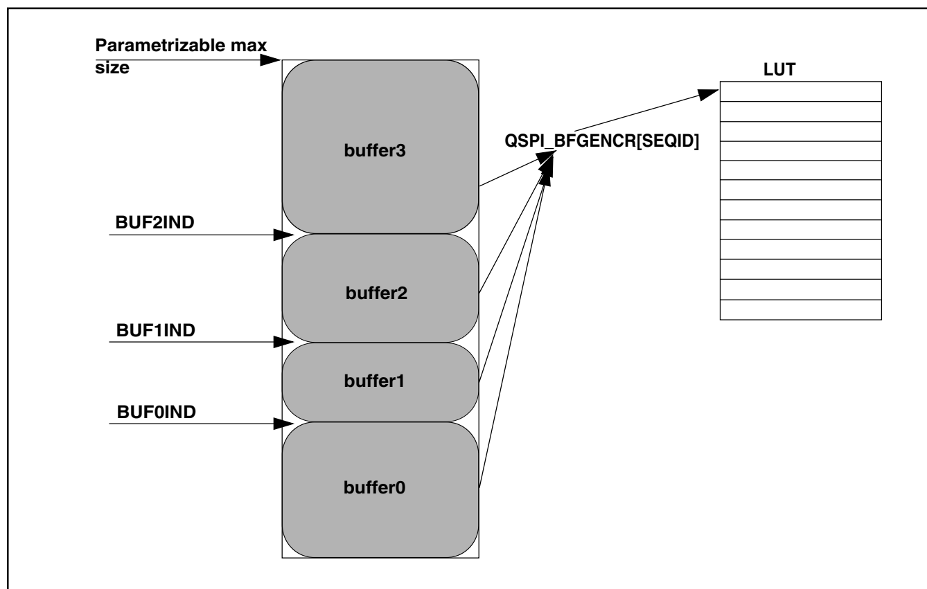
Figure 35-4. Flexible AHB Buffers
