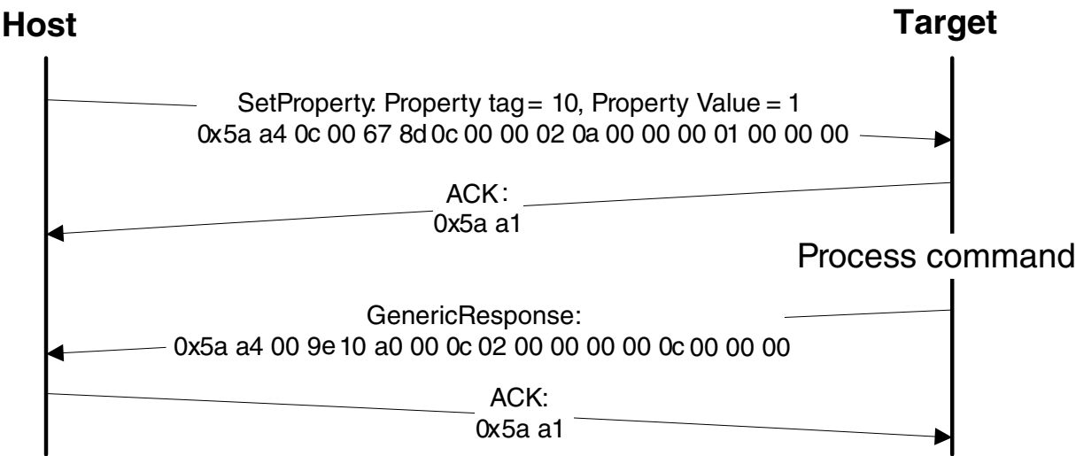
Figure 14-11. Protocol Sequence for SetProperty Command
