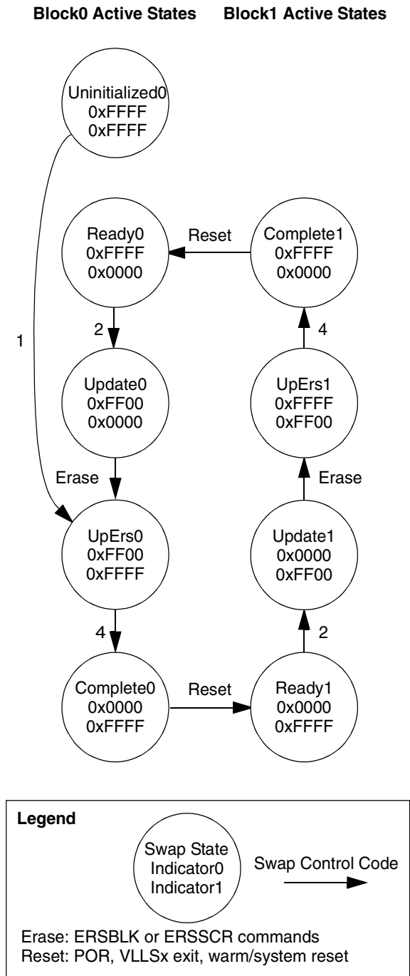
Figure 33-7. Valid Swap State Sequencing
