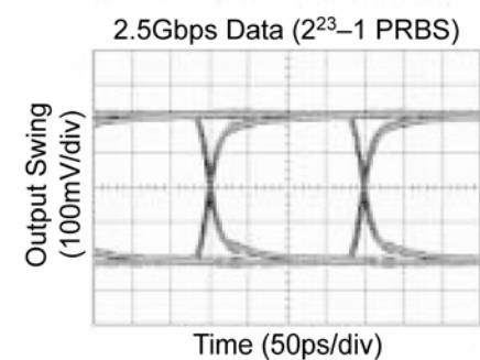
2^{23}-1 PRBS Pattern
