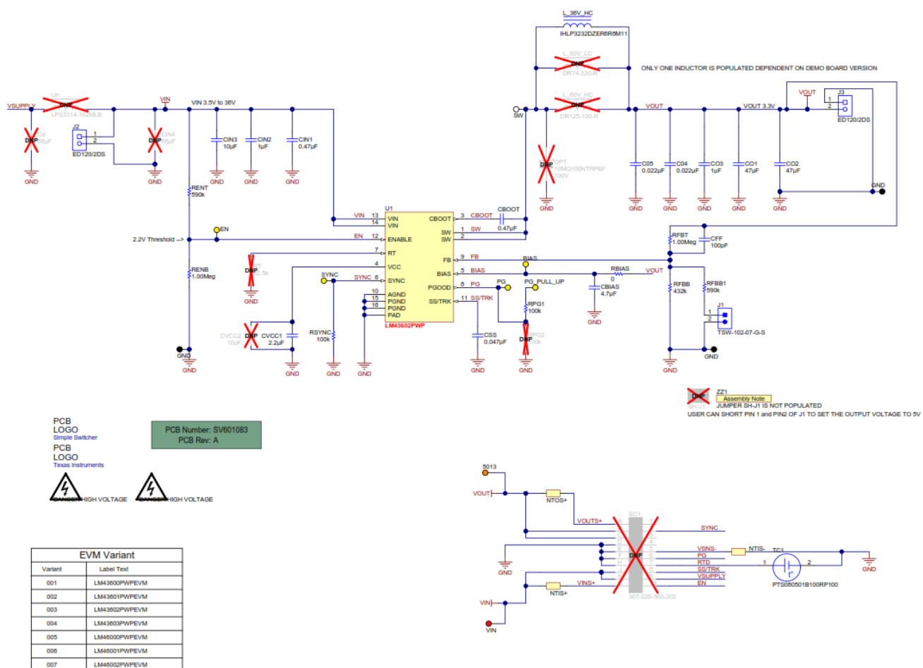
Figure 2. LM43602EVM Schematic
