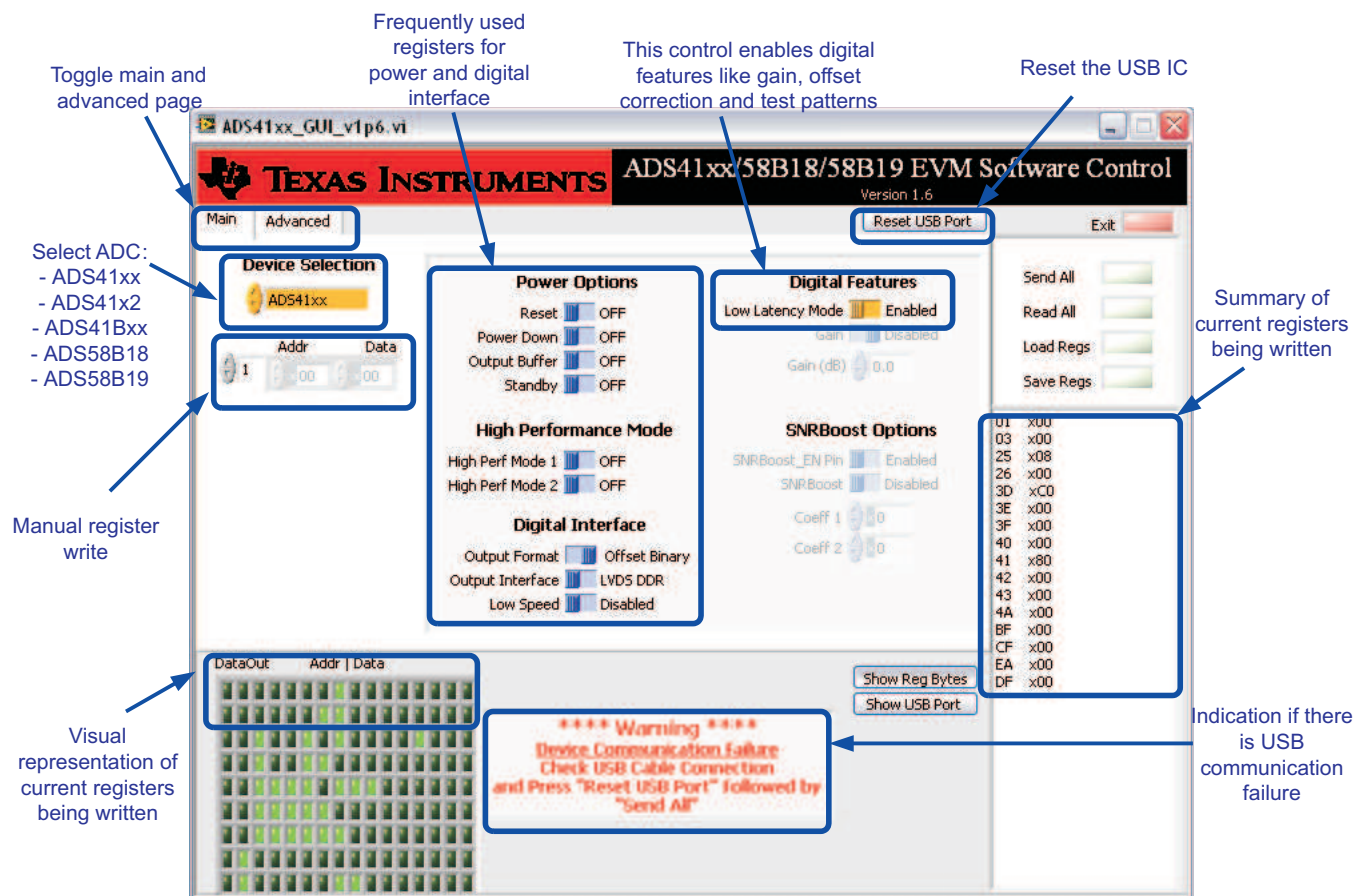
Figure 6. GUI Main Page
