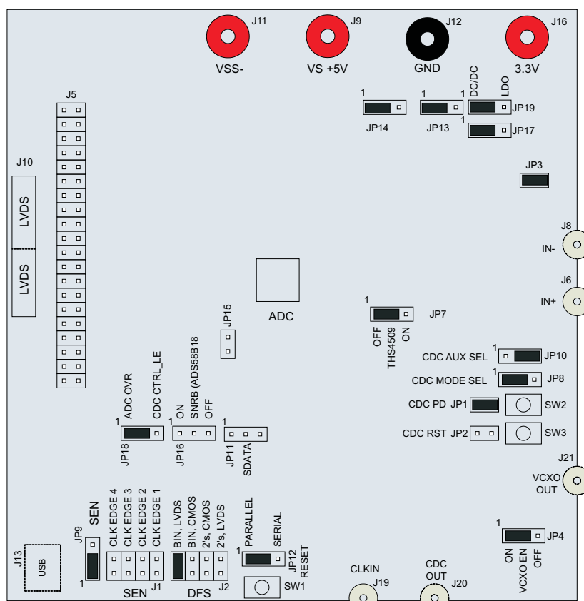
Figure 1. ADS41xx Jumpers
