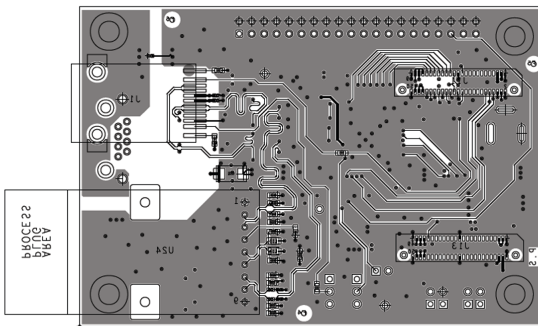
Figure 18. Layer 4 - Signal
