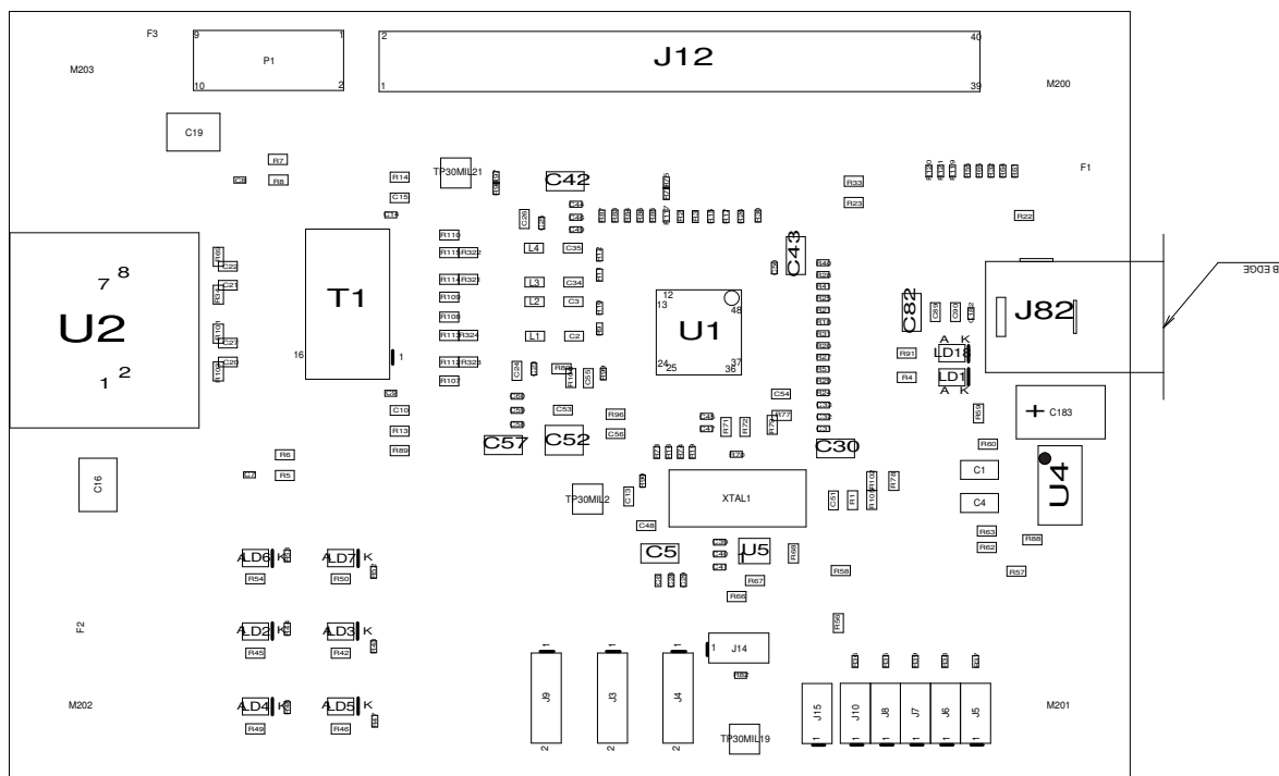
Figure 19. Layer 1 – Components Side Assembly
