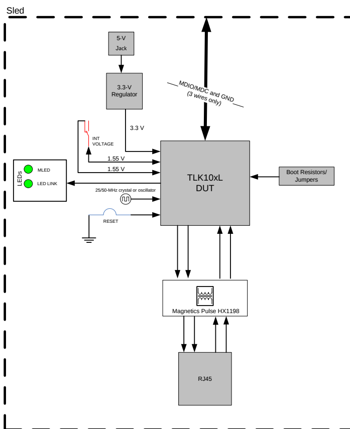
Figure 2. MDIO/MDC Interface Block Diagram
