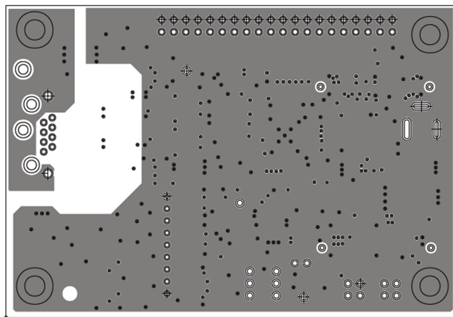
Figure 16. Layer 2 - GND
