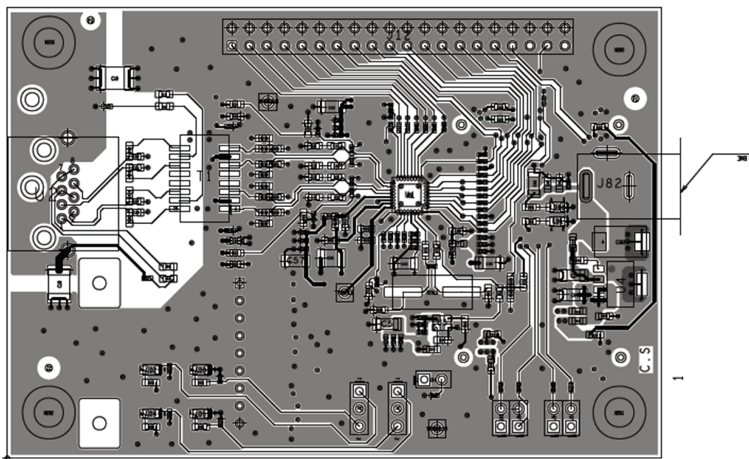
Figure 15. Layer 1 - Signal
