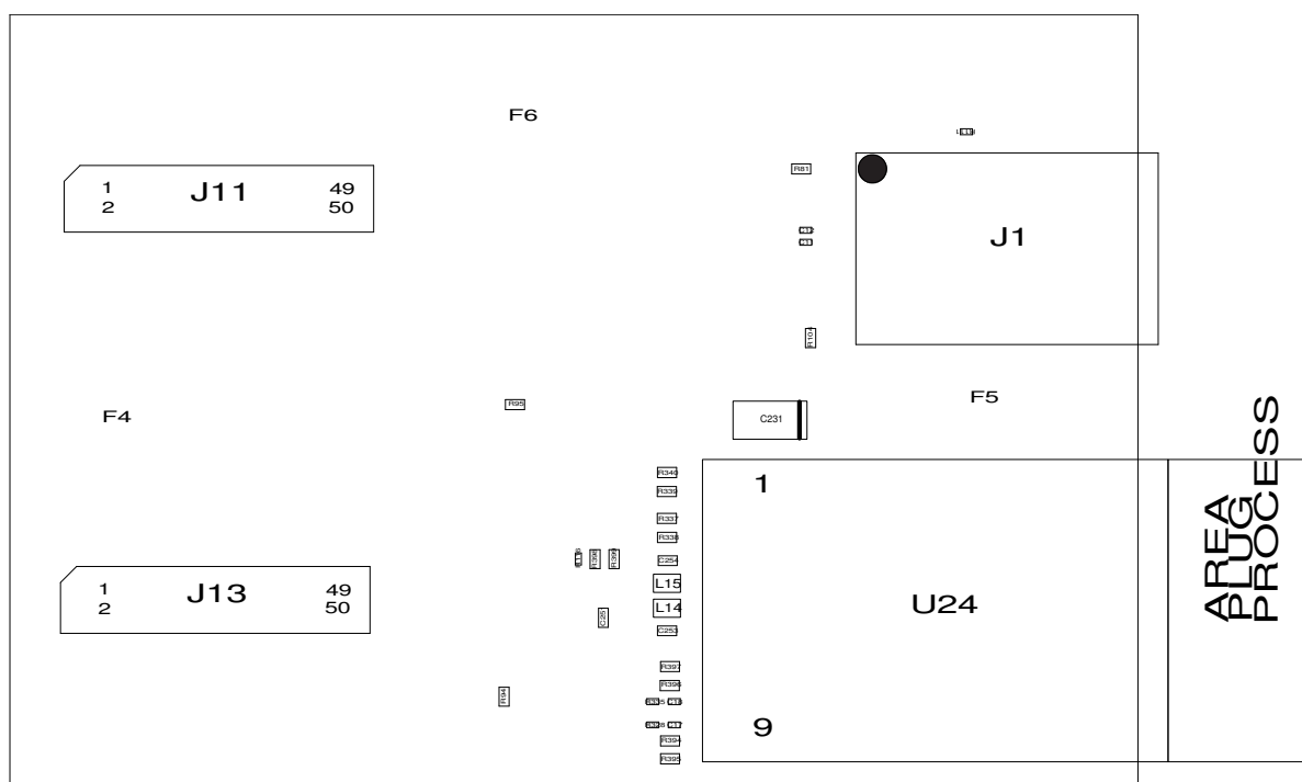
Figure 20. Layer 4 – Print Side Assembly
