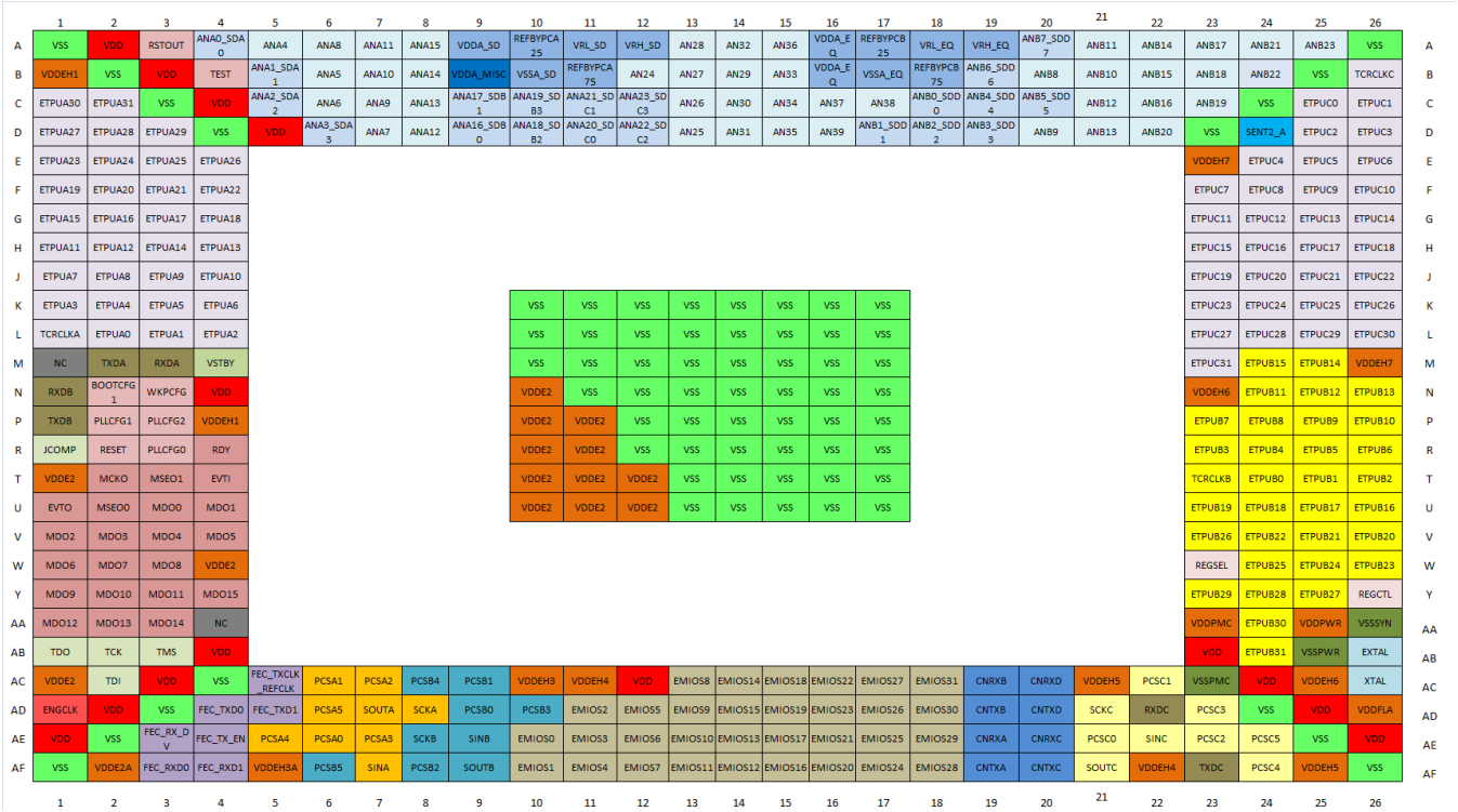
Figure 2. MPC5775E 416-ball MAPBGA (full diagram)
