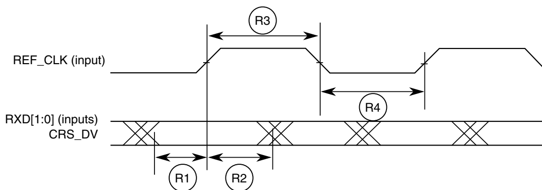
Figure 40. RMII receive signal timing diagram
