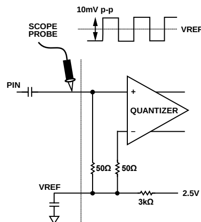
Figure 24. Single-Ended Sensitivity Measurement
