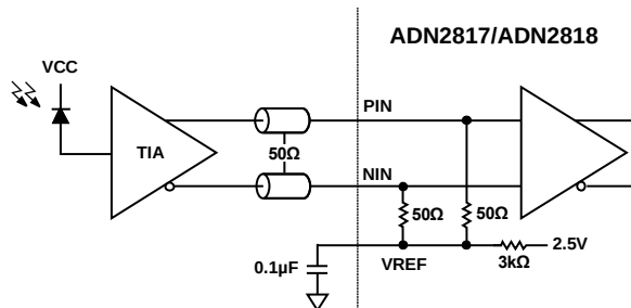
Figure 40. DC-Coupled Application
