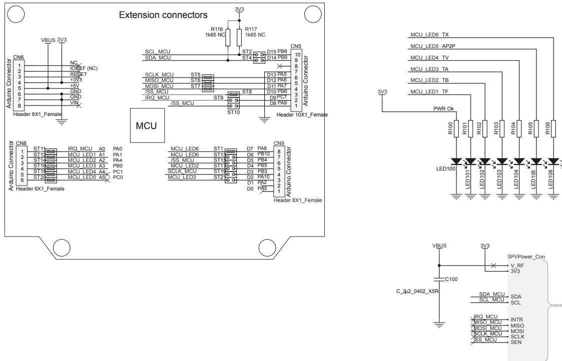
Figure 4. X-NUCLEO-NFC06A1 circuit schematic (2 of 3)
