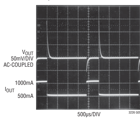
LDO Output Transient Step Response Waveform
